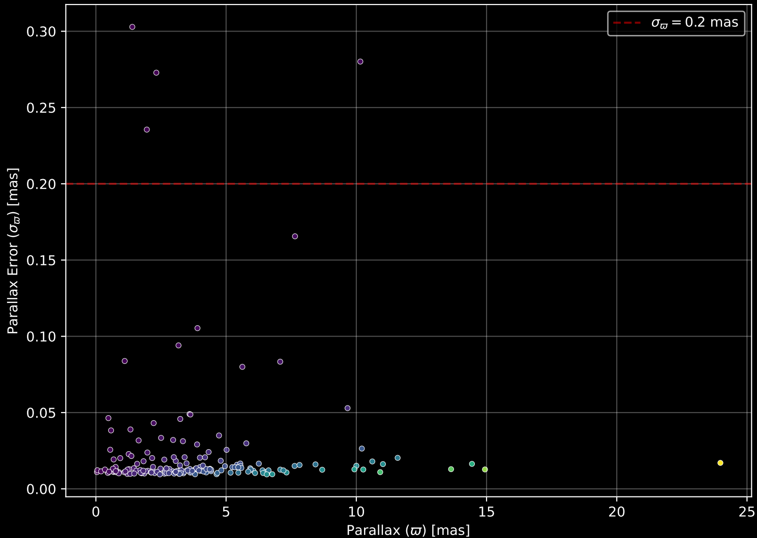
APOGEE DR17 Field: [115+64_MGA] Parallax Quality (n= 188)
