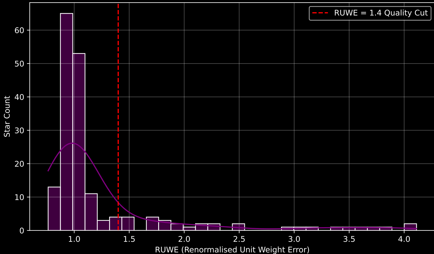
GAPOGEE DR17 Field [115+64_MGA] RUWE Distribution (n= 179)
