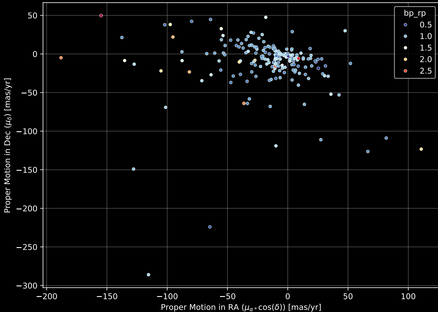
APOGEE DR17 Field: [115+64_MGA] Proper Motion Diagram (n= 188)
