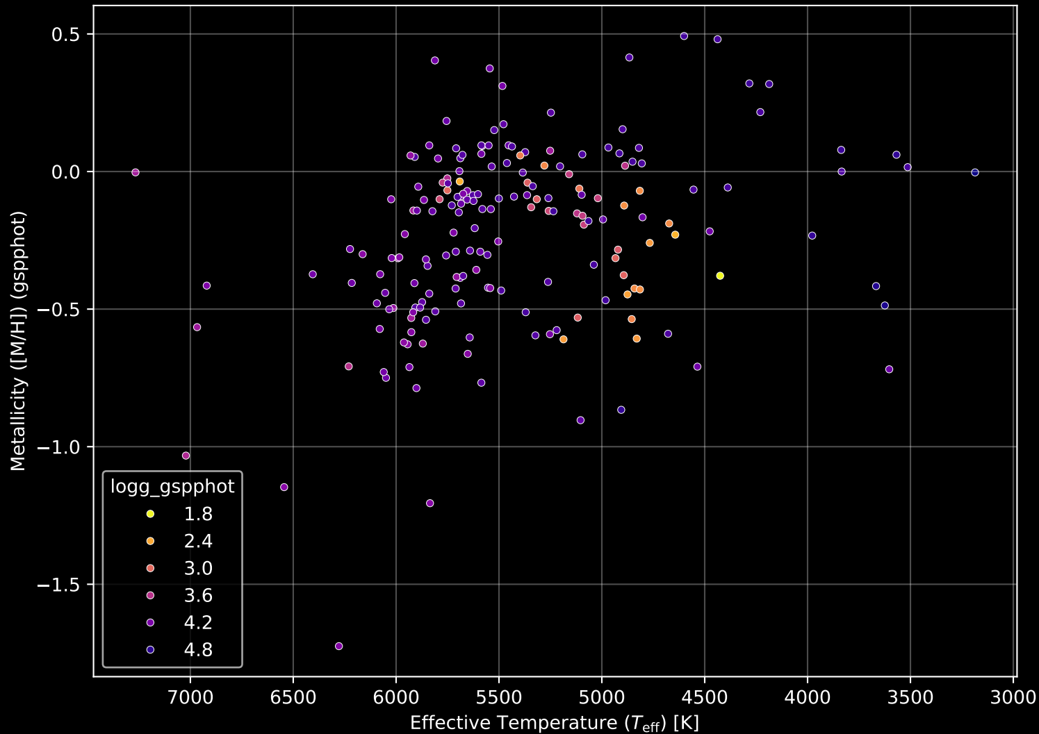
APOGEE DR17 Field: [115+64_MGA] Stellar Population Parameters (n= 188)
