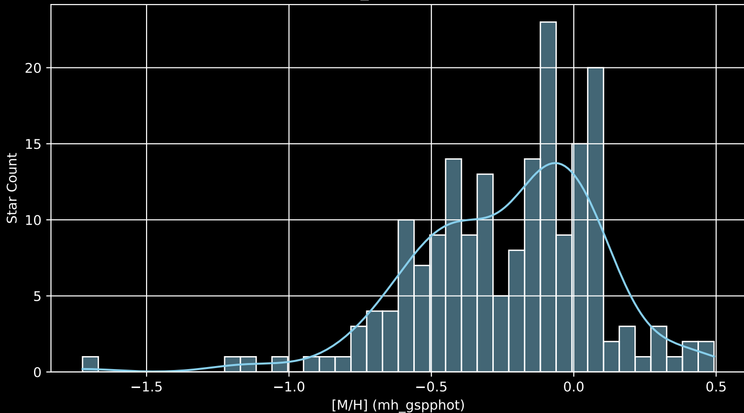
APOGEE DR17 Field: [115+64_MGA [M/H] (mh_gspphot) (n= 188)
