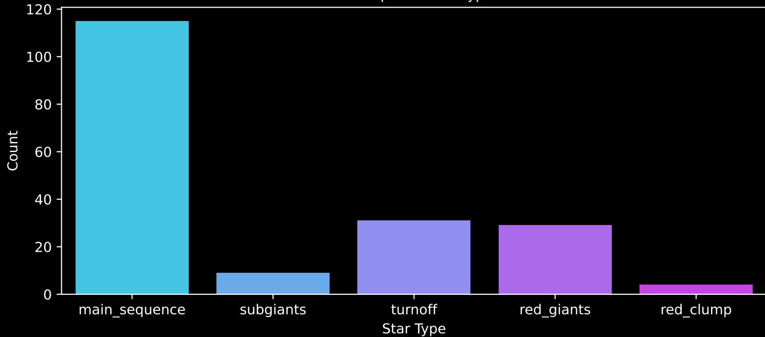
APOGEE DR17 Field: [115+64_MGA] Count plot of Star Type
