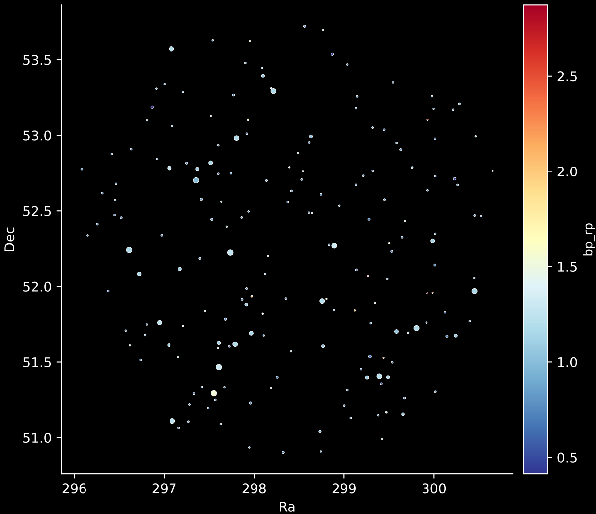
APOGEE DR17 Field: [115+64_MGA] Stars: 188
